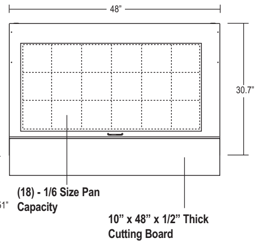
CRMR48-18M PLAN VIEW
