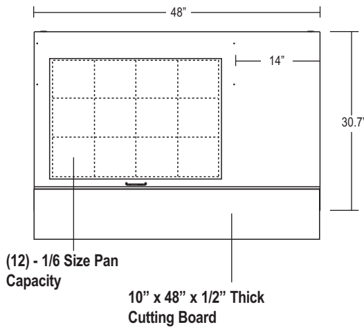
CRMR48-12M PLAN VIEW
