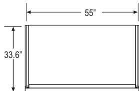
PLAN VIEW
